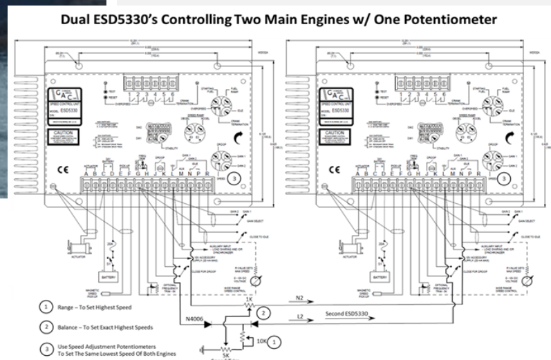
Wiring Diagram
