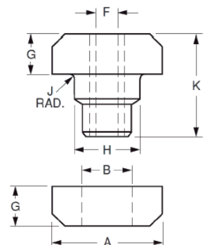
SR128 Vibration Dampeners
